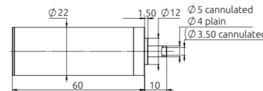
22 MM MOTOR
